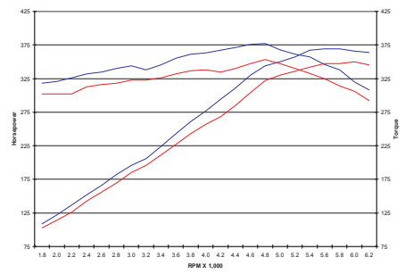
2006-07 Chrysler 300 / Dodge Charger / Magnum SRT8 6.1L Ultra Flo Welded Kit - 19440 26 HP, 32 lbs. ft @4200 RPM
