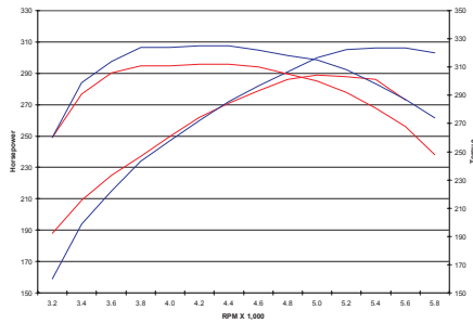
1998-2002 Chevy Camaro / Pontiac Firebird / Trans Am 5.7L Ultra Flo Bullet Kit - 19418 32 HP, 28 lbs. ft @6000 RPM
