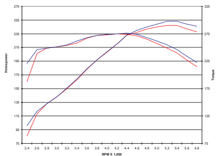
2007 Chevy Tahoe / GMC Yukon 5.3L Ultra Flo Welded Kit - 19436 15 HP, 33 lbs. ft @ 2400 RPM
