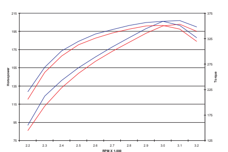
2001-06 Silverado / Sierra 2500 HD/3500 6.6L Duramax Diesel Ultra Flo Welded Kit - 19375 11 HP @2300 RPM, 15 ft lbs. ft 3400 RPM
