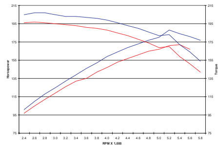
2005-07 Ford Mustang V6 4.0L Ultra Flo Welded Kit - 19434 17 HP, 13 lbs. ft @ 5400 RPM
