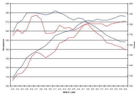
2005-07 Chrysler 300 / Dodge Charger / Magnum 3.5L Super Turbo Kit - 19422 17 HP, 21 lbs. ft @4100 RPM
