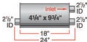
Camaro/Firebird 17266 Street - 573 260/520
